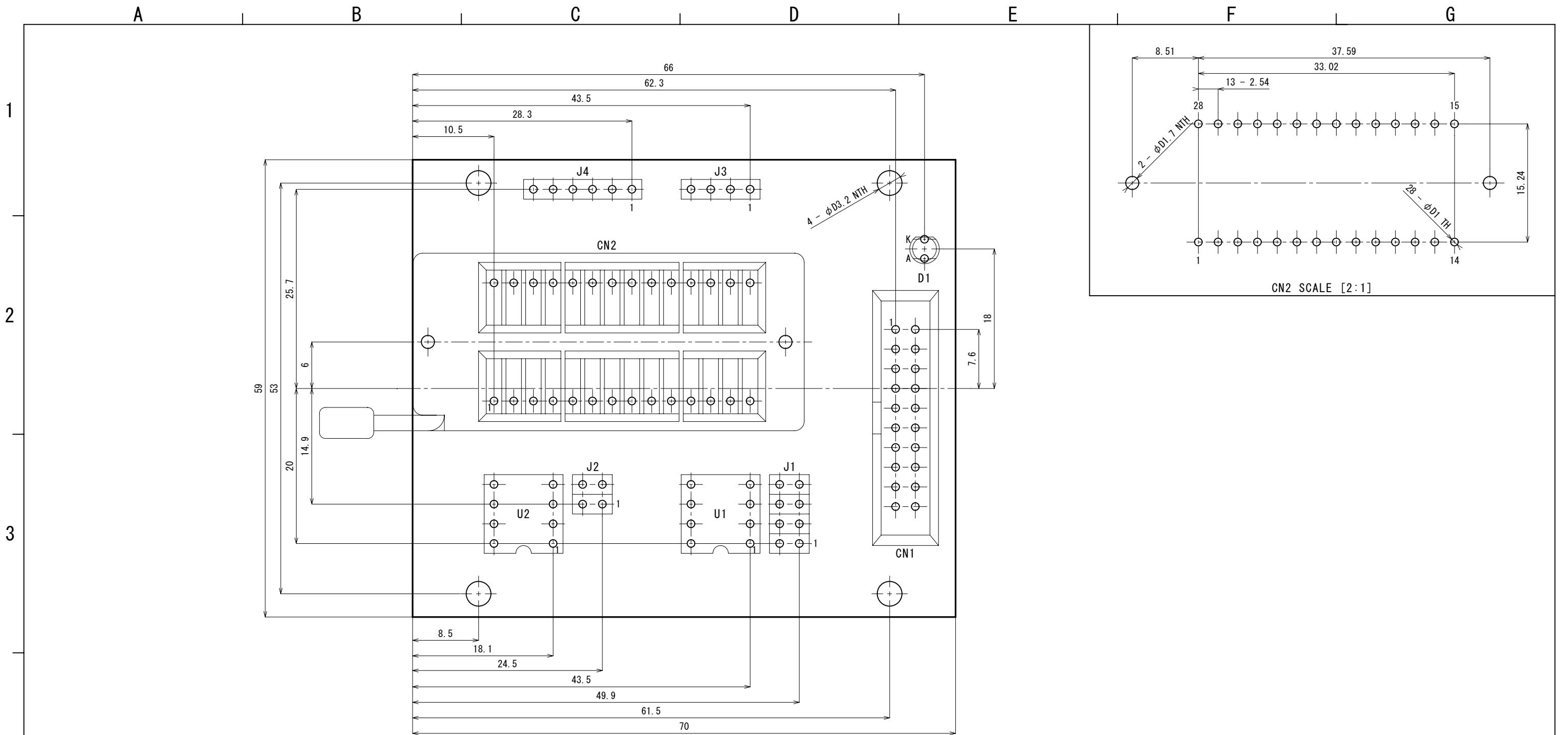
COMPONENT SIDE [TOP VIEW]
